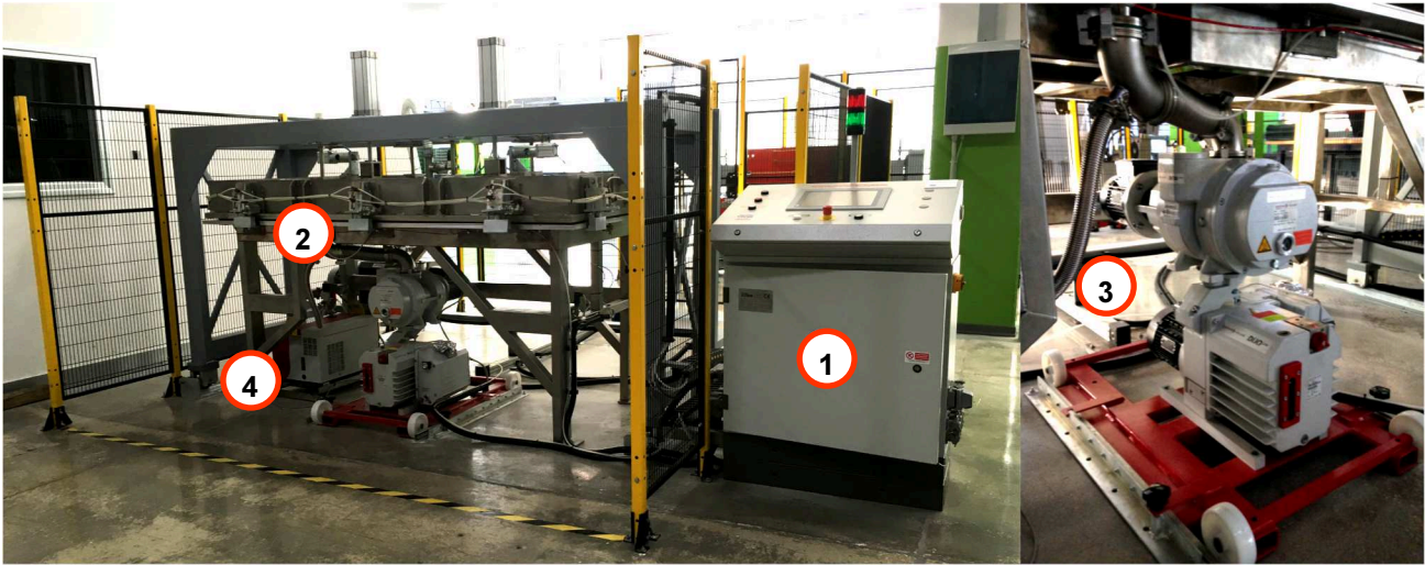
1. Control Station 2. Vacuum Test Chamber 3. Vacuum Pump and Blower 4. Helium Mass-Spectrometer
